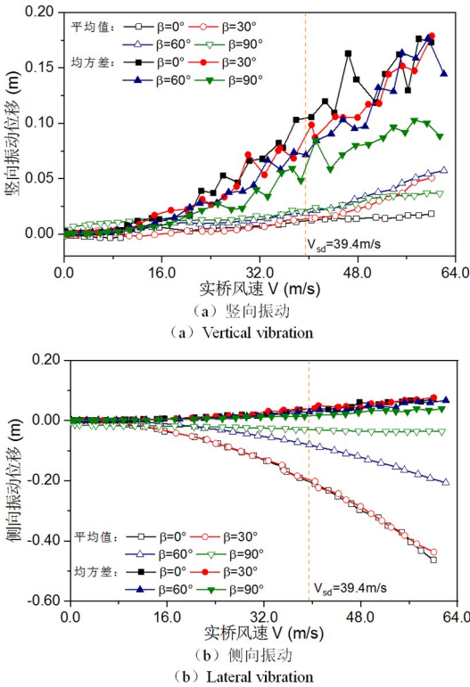
图 10 不同风偏角下钢导梁悬臂端振动位移随风速变化 Fig. 10 Vibration displacements of the launching nose tip under various wind yaw angles versus wind velocity
