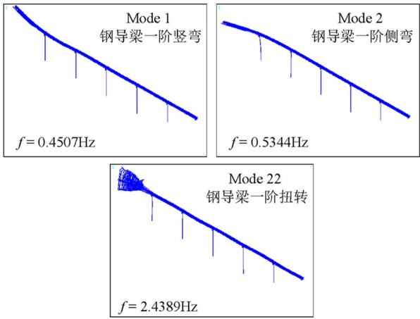
图4 顶推施工期主桥关键模态振型 Fig.4 Key mode shapes of the bridge at launching
