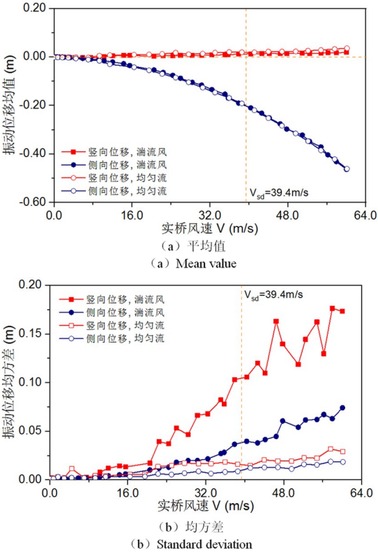
图 9 紊流风和均匀流下钢导梁悬臂端振动位移随风速变化 Fig. 9 Vibration displacements of the launching nose tip versus wind velocity in turbulent and smooth flows
