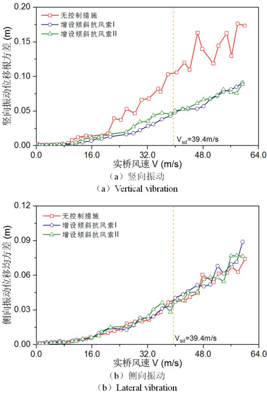
图 13 有无倾斜抗风索的钢导梁悬臂端振动位移随风速变化 Fig. 13 Vibration displacements of the launching nose tip with and without the inclined wind-resistance cables
