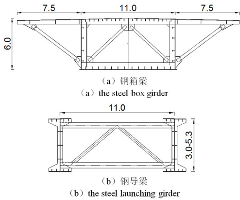
图2 钢箱梁和钢导梁标准横断面图(单位:m) Fig.2 Cross sections of the box girder and launching girder
