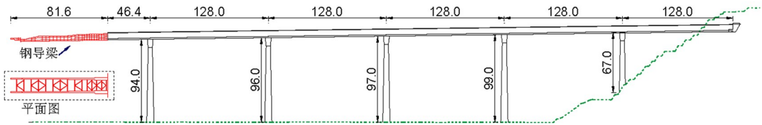
图1 顶推施工期主桥立面布置(单位:m) Fig.1 General elevation of the bridge at launching
