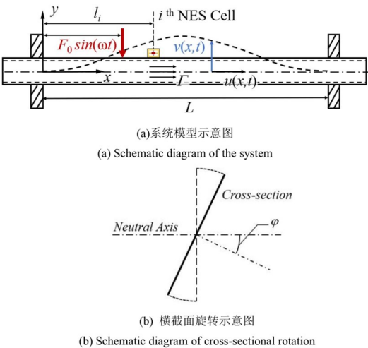
图 1 安装非线性能量汇胞元的输流管道系统模型和管道横截面旋转的示意图 Fig. 1 The schematic diagram of model in the fluid-conveying pipe with nonlinear energy sink cells and the cross-sectional rotation of the pipe
