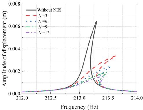
图 4 不同数量胞元下系统的幅频响应曲线 Fig. 4 The amplitude-frequency response curves of the system under different numbers of NES cells
