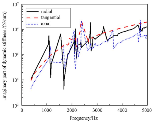
图 3 阻尼器的动刚度曲线 Fig. 3 Dynamic stiffness curve of damper
