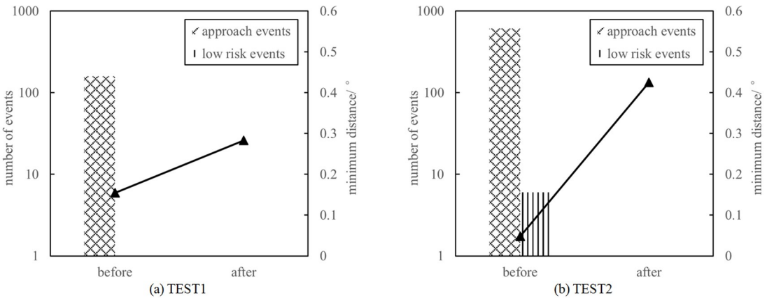
图 5 倾角微调后的碰撞风险变化 Fig. 5 Changes of collision risk after fine-tuning inclination
