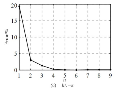
Fig. 3 The relative error of calculated sound pressure corresponding to different wave functions
