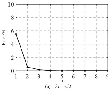
Fig. 3 The relative error of calculated sound pressure corresponding to different wave functions
