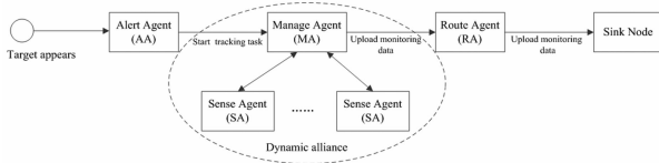
图 12 基于多智能体系统的无线传感器网络目标跟踪控制框架 Fig. 12 Target tracking control frame of wireless sensor network based on multi - agent system
