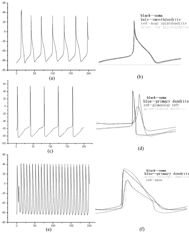
图2 (a)、(c)和(e)依次为在直流电刺激0.25nA作用在胞体处时浦肯野神经元、僧帽神经元和CA1锥体神经元的胞体电位发放图，(b)、(d)和(f)依次为上述三种神经元对应的各部分电位图 Fig. 2 (a)、(c) and (e) are soma action potential of purkinje neuron, mitral neuron and CA1 pyramidal neuron under DC stimulation of 0.25nA on soma respectively; (b)、(d) and (f) are each part's action potential of three principal neurons mentioned above
