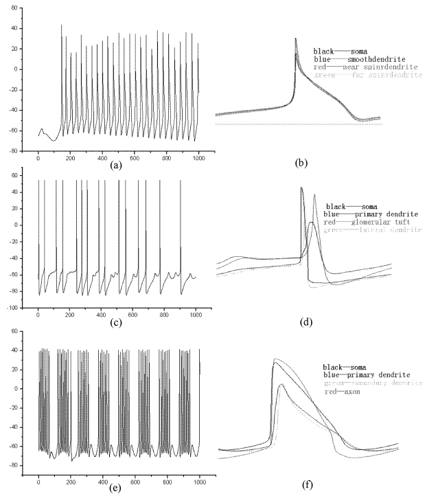
图3 (a)、(c)和(e)依次为交流电刺激0.12+0.18sin(0.05t)nA作用在胞体处时浦肯野神经元、僧帽神经元和CA1锥体神经元的胞体电位发放图,(b)、(d)和(f)依次为上述三种神经元对应的各部分电位图 Fig. 3 (a)、(c) and (e) are soma action potential of purkinje neuron, mitral neuron and CA1 pyramidal neuron under AC stimulation of 0.12 + 0.18sin(0.05t) nA on soma respectively; (b)、(d) and (f) are each part's action potential of three principal neurons mentioned above
